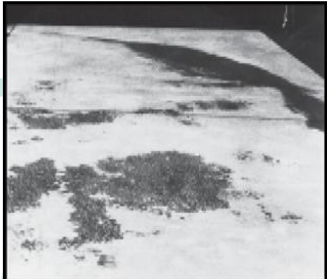
Discoloration on a Slab on Ground
